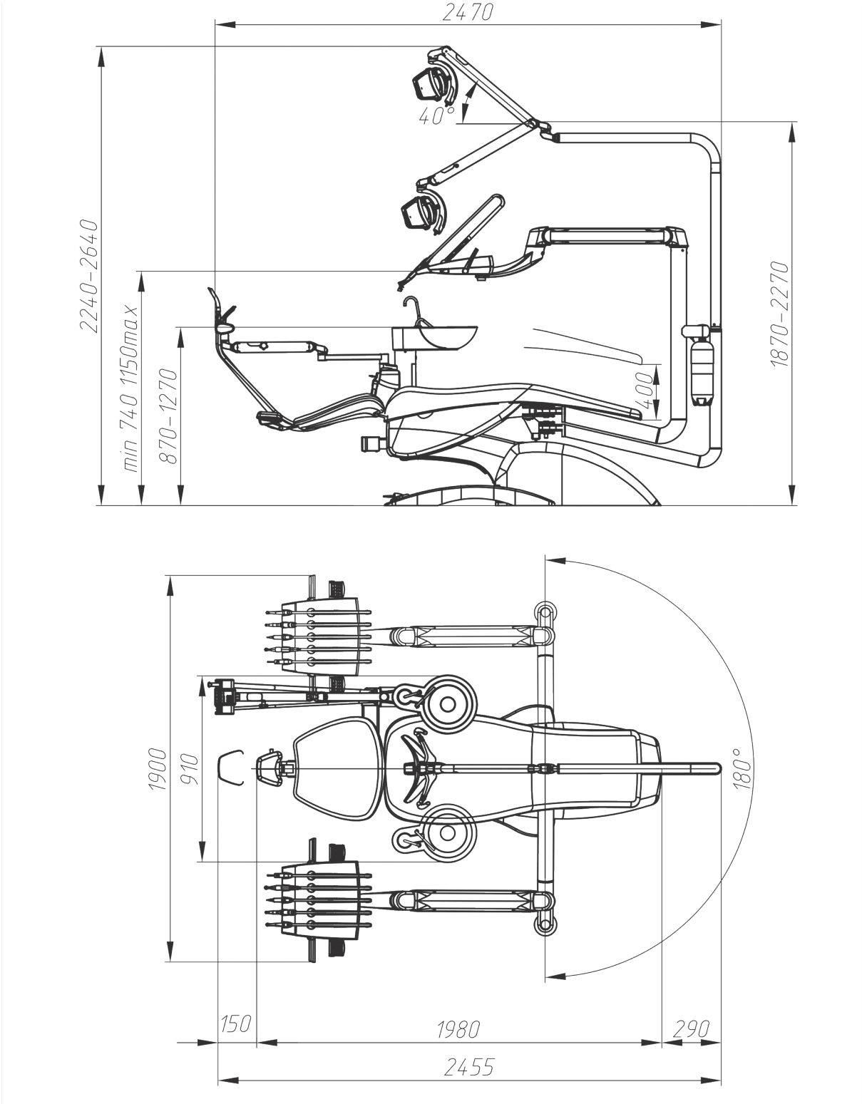
Overall dimensions of GALIT AMBIDEXTRE dental unit with upper delivery of instruments and STING patient chair.
