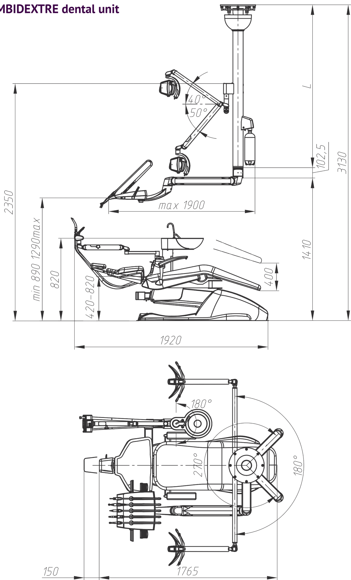
Overall dimensions of Galit AMBIDEXTRE dental unit: with the dentist console attachment to ceiling and with 2009 NEXT patient chair.
