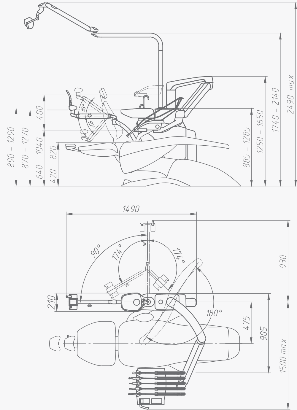
Overall dimensions of hanging dental unit GALLANT OMNIPRATIQUE with upper delivery of instruments and patient chair STING
