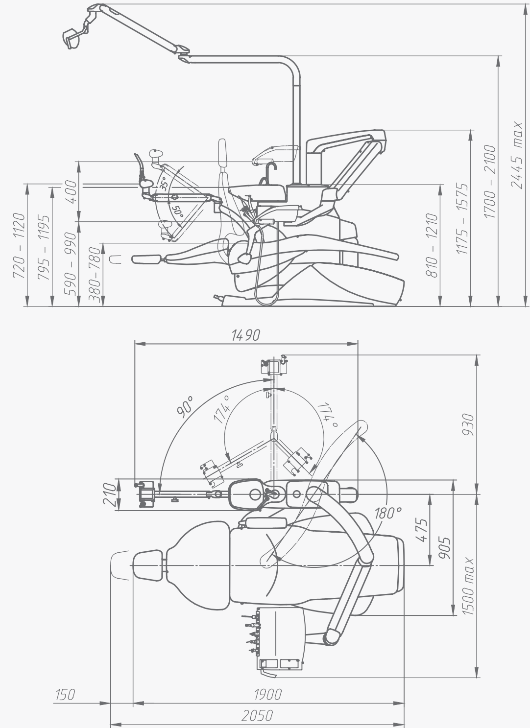
Overall dimensions of hanging dental unit GALLANT OMNIPRATIQUE with lower delivery of instruments and patient chair ECO NEXT.
